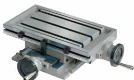
MB2 Cross table. X = 280 mm. Y = 180 mm. Table net weight = 40 kg. Available for Z/X series.
